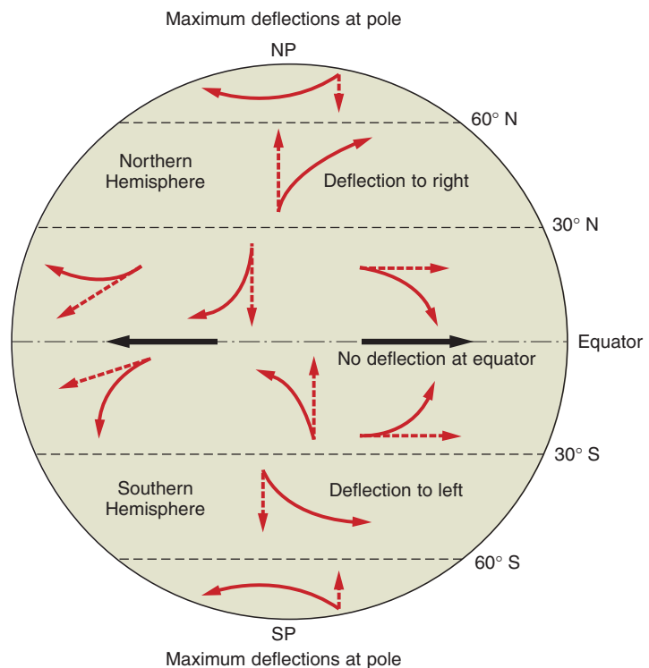
FIGURE 5.6 Schematic illustration of the apparent deflection (Coriolis effect) of an object caused by Earth’s rotation when an object (or the wind) moves north, south, east, or west in both hemispheres.
