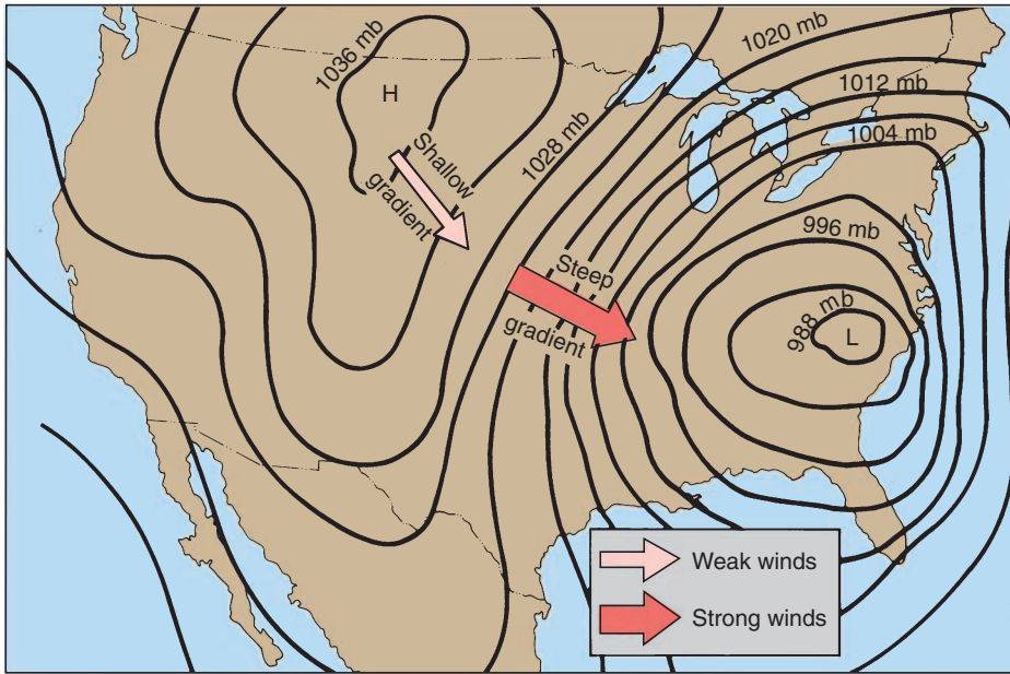
FIGURE 5.5 The relationship of wind to the pressure gradient: The steeper the pressure gradient, the stronger will be the resulting wind. Where else on this figure (other than the area indicated) would winds be strong?
