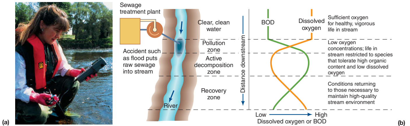
FIGURE 19.2 (a) Pollution-control officer measuring oxygen content of the River Severn near Shrewsbury, England. (b) The relationship between dissolved oxygen and biochemical oxygen demand (BOD) for a stream after the input of sewage.
