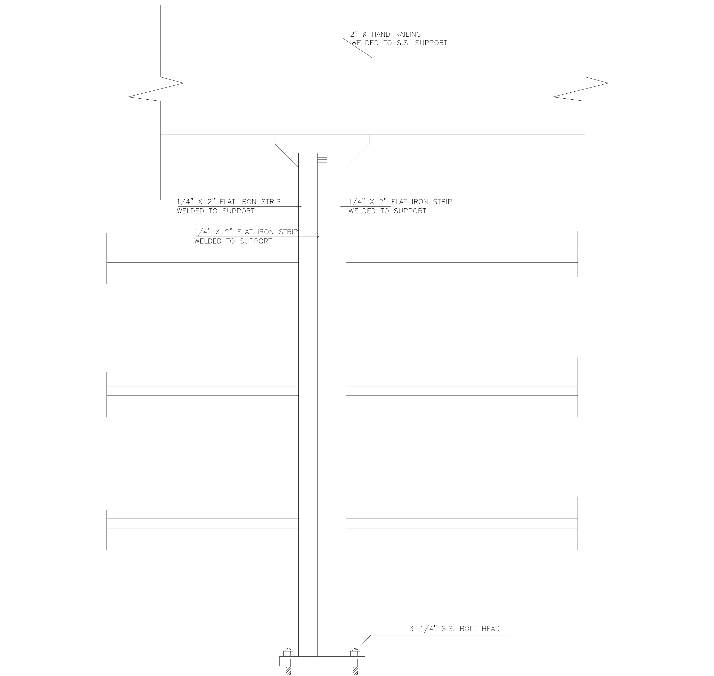
HAND RAIL FRONT ELEVATION
