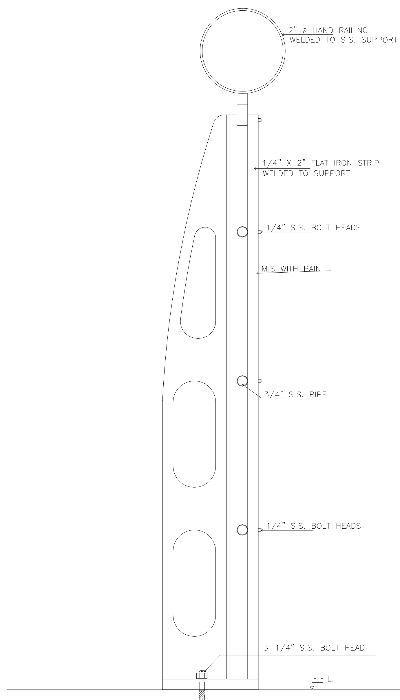
HAND RAIL SITE ELEVATION
